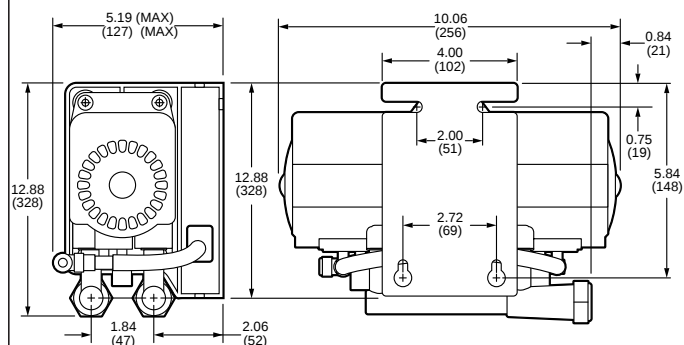
Dual Pump (Model G257xxx)
