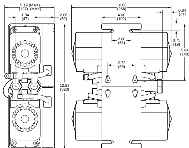
Quatro Pump (Model G457xxx)
